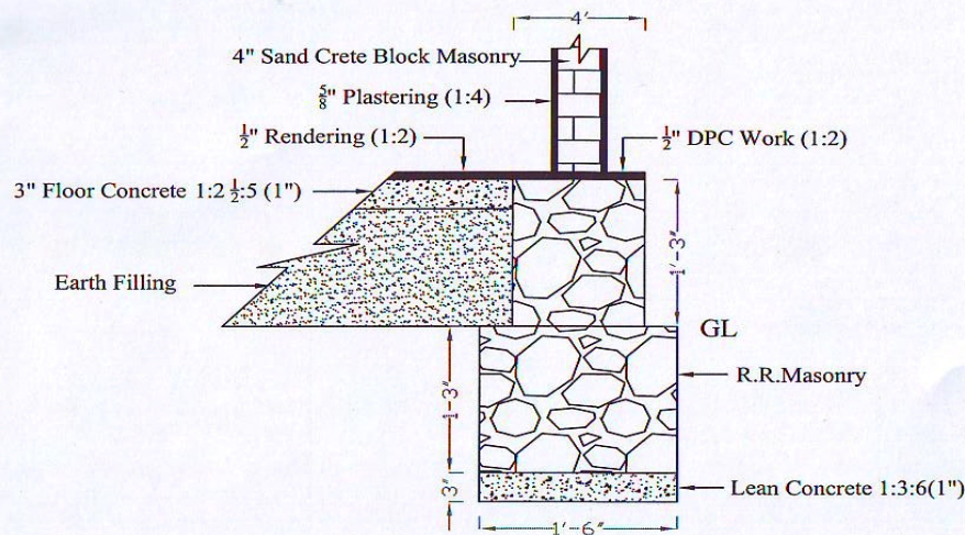
WALL FOUNDATION WITHOUT PLINTH BEAM
