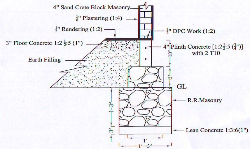
WALL FOUNDATION WITH PLINTH BEAM
