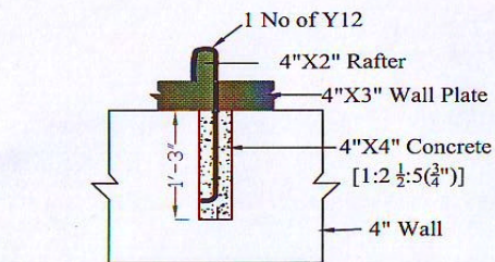
JOINT OF RAFTER & WALL PLATE WITH WALL
