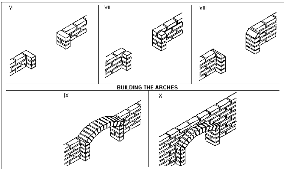
Fig. 218: Building the butressed reveals of the openings. Note the thickness of the arch on the outside.
