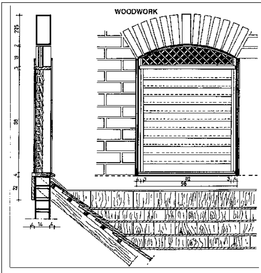
Fig. 278: Elevation and vertical section of a «nacos» window with fretwork impost, on the first floor.
