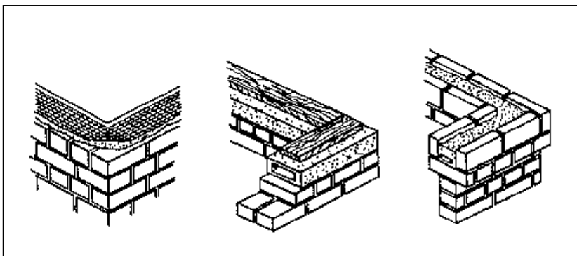
Fig. 120: Ring-beams and reinforced comers using wood or steel embedded in the wall.
