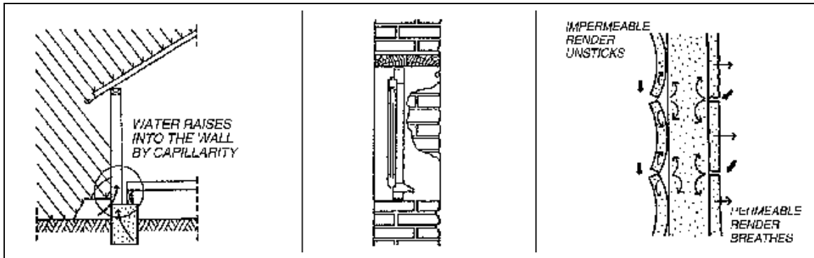
Fig. 74: Problems of humidity at the base of walls.
