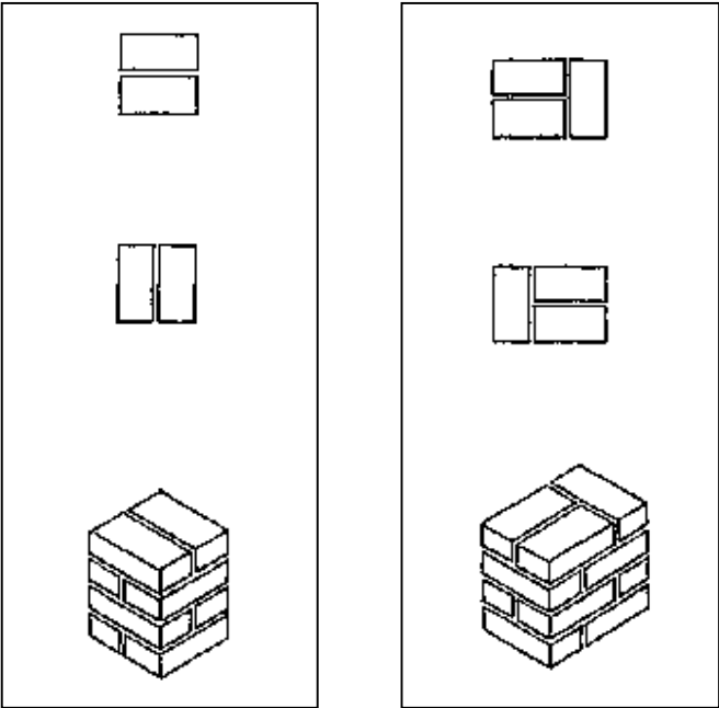
Fig. 59 a: Simple bonding pattern for a 30 cm pillar. Fig. 59 b: Simple bonding pattern for a 30x45 cm pillar.
