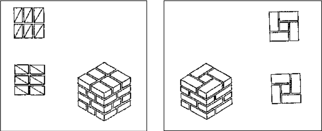
Fig. 61 a: Classic bonding pattern for a 45 x 45 cm pillar. Fig 61 b: Simplified bonding pattern for a 45 x 45 cm pillar.
