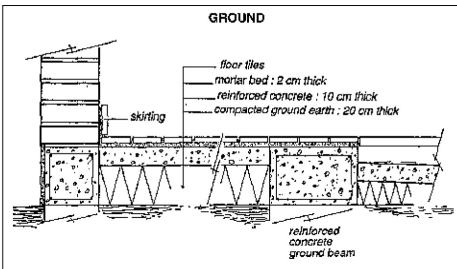
Fig. 327: Detail of working drawing for foundations.
