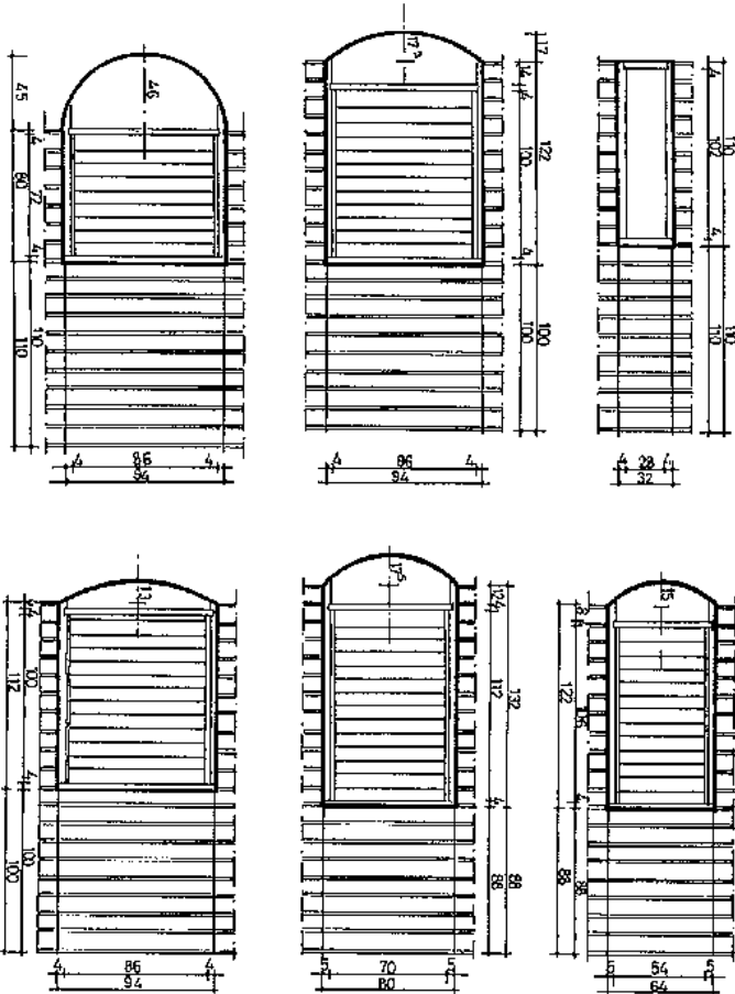
Fig. 277: Drawings of the complete range of door and window openings with Dutch or semi-circular arches.
