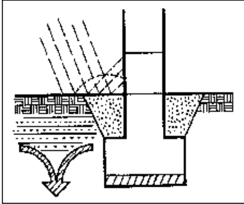
Fig. 86: Infiltration without accumulation.
