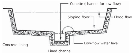
Open-channel drain for wastewater and storm-water 57
